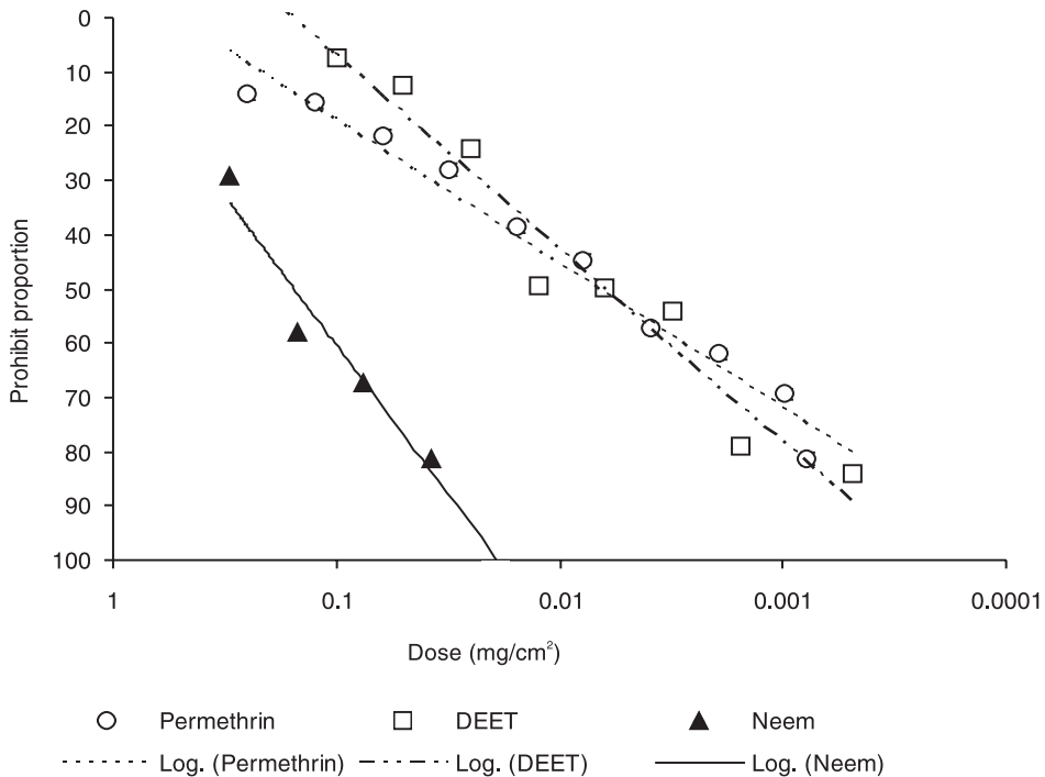
Figure 1 Probit regression line of permethrin, DEET and neem against a laboratory strain of Anopheles stephensi
