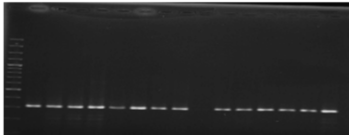
Figure 1 Two PCR assays confirm identification of Anopheles arabiensis as the sole member of An. gambiae complex in greater Khartoum. Lane 1: 100 kb molecular markers; lanes 2, 3, 4: Shambat and Eltamanyat samples; lanes 5, 6, 7: Soba West; lanes 8, 9: Almaygoma; lane 10: negative control; lanes 11, 12: Alhaj Yousif; lanes 13,14: Alshegalab; and lanes 15, 16: Arkewit
