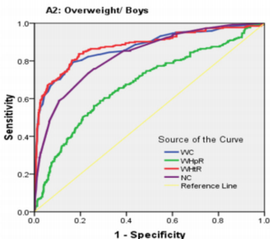
Figure 2 Area under the receiver operating characteristic curves for waist circumference (WC), waist-to-hip ratio (WHpR), waist-to-height ratio (WHtR) and neck circumference (NC) to define overweight in females (A1) and males (A2), and obesity in females (B1) and males (B2)
