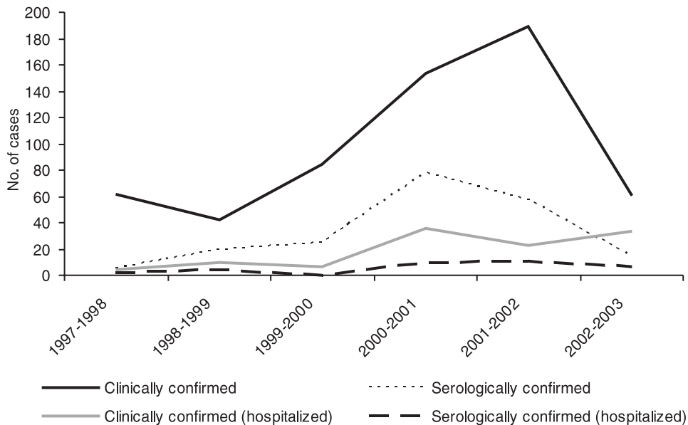
Figure 1 Number of clinically diagnosed measles cases with serum specimens, serologically confirmed cases and hospitalized cases, Ghazvin district, April 1997–April 2003
