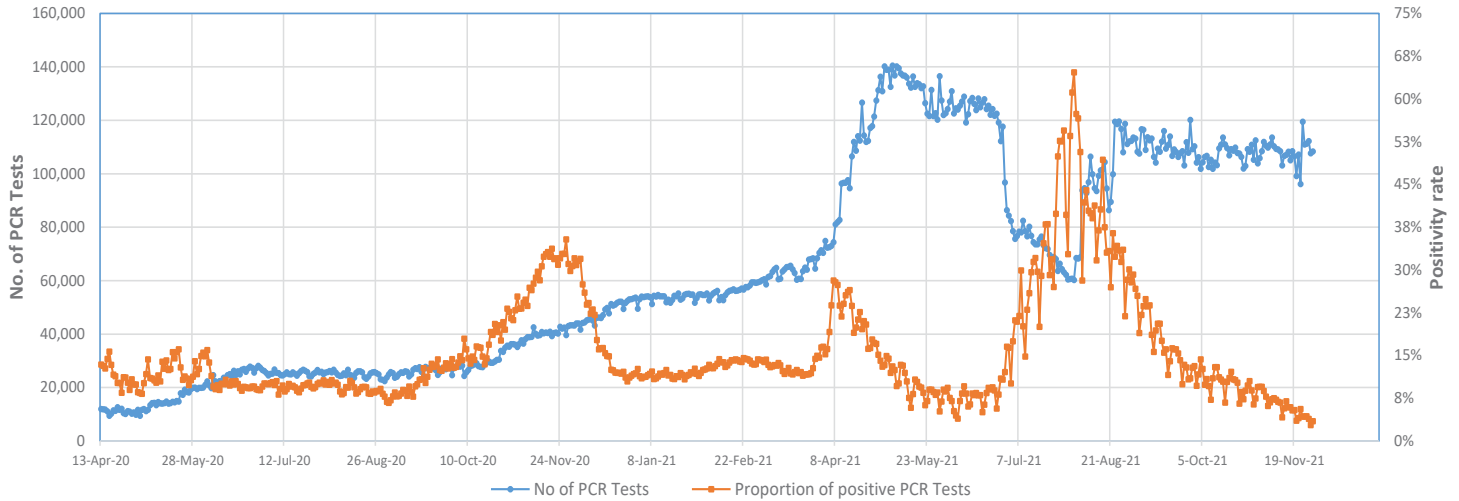
Figure 3 - Number of Daily COVID-19 PCR Tests and Percentage of Positive Cases, 13 April 2020 - 28 November 2021
