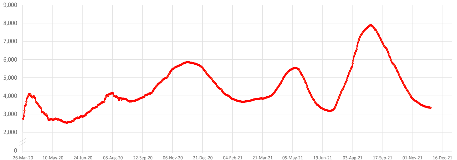
Figure 2 - COVID-19 Patients in Intensive Care, 26 March 2020 - 28 November 2021
