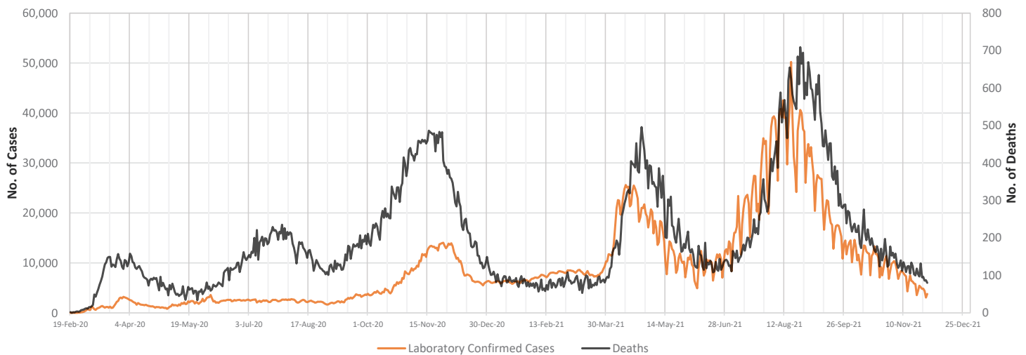
Figure 1 - Trend of COVID-19 Laboratory-Confirmed Cases and Deaths, 19 February 2020 - 28 November 2021
