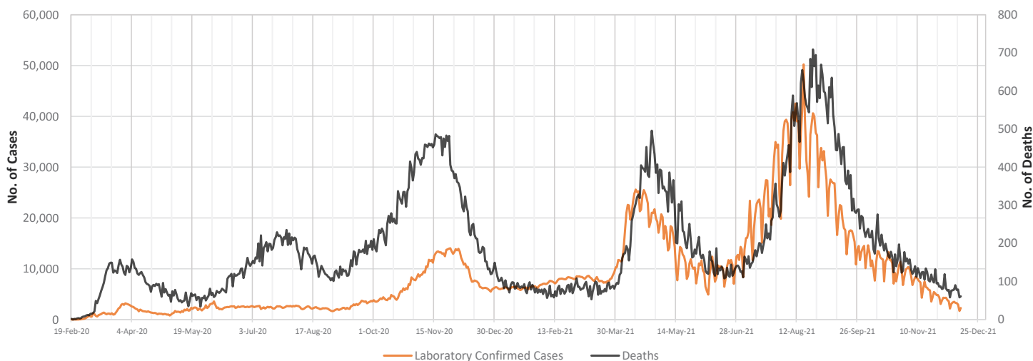
Figure 1 - Trend of COVID-19 Laboratory-Confirmed Cases and Deaths, 19 February 2020 - 12 December 2021
