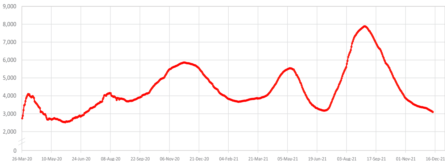
Figure 2 - COVID-19 Patients in Intensive Care, 26 March 2020 - 12 December 2021
