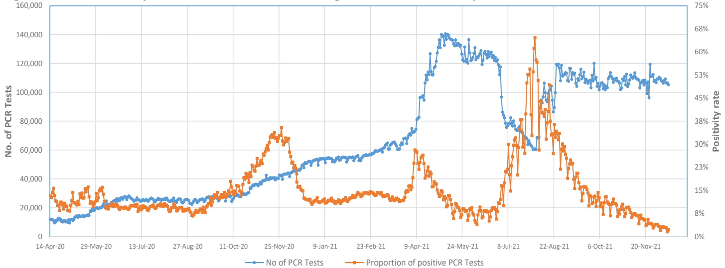
Figure 3 - Number of Daily COVID-19 PCR Tests and Percentage of Positive Cases, 13 April 2020 - 12 December 2021
