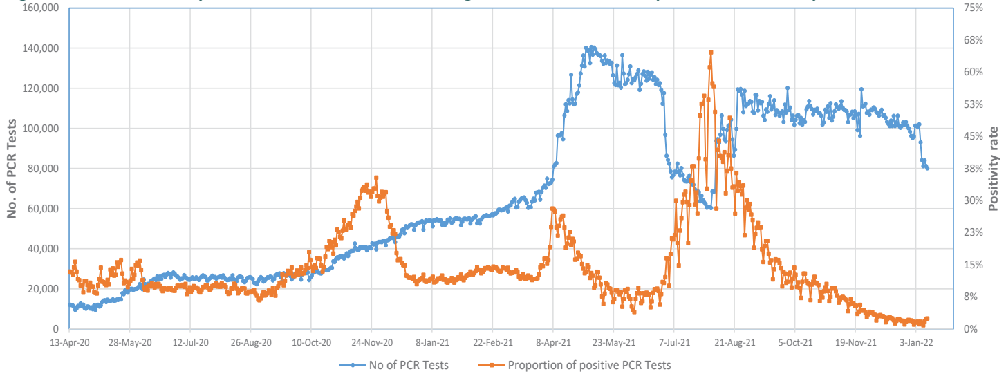
Figure 3 - Number of Daily COVID-19 PCR Tests and Percentage of Positive Cases, 13 April 2020 - 11 January 2022
