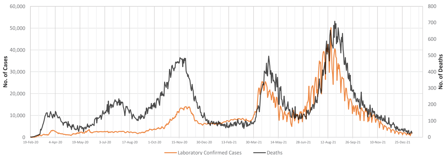
Figure 1 - Trend of COVID-19 Laboratory-Confirmed Cases and Deaths, 19 February 2020 - 11 January 2022
